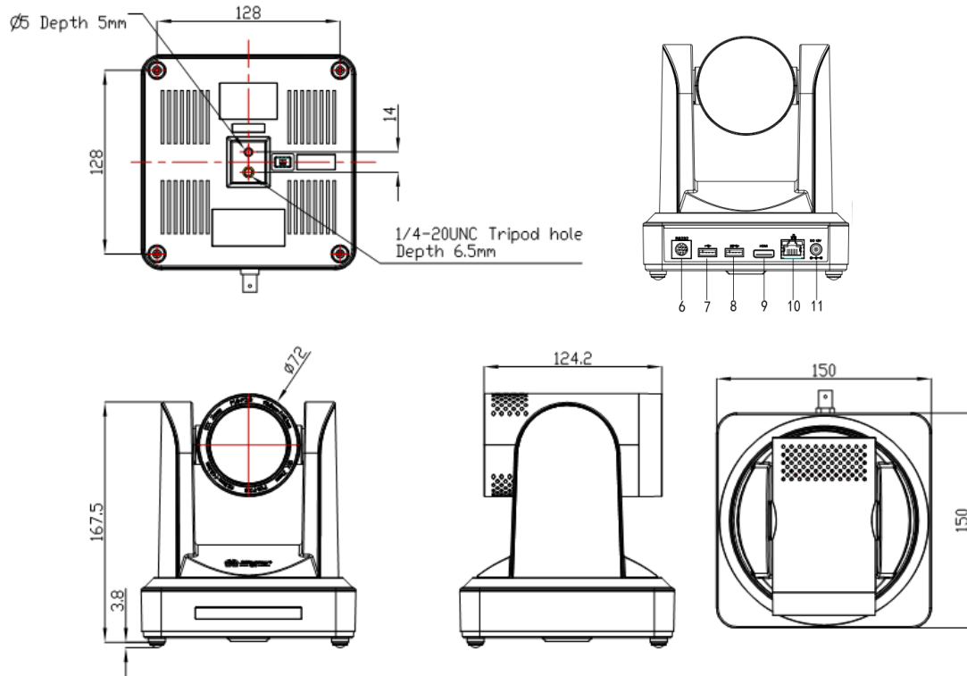
Figure 2.2 Camera dimension
